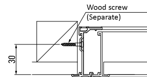
Wood framing detail drawing
