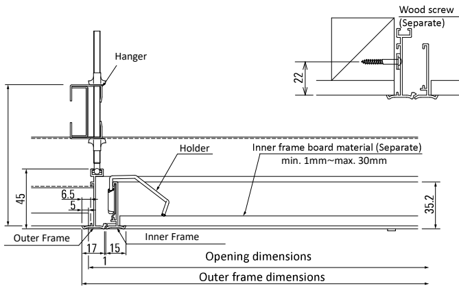
Detail Drawing
