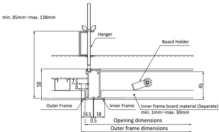
Detail Drawing
