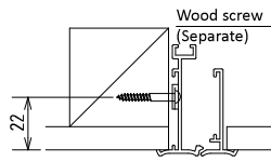
Wood framing detail drawing
