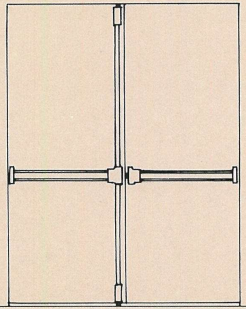
DOUBLE LEAF DOOR: 1 side latch type device and 1 top and bottom latch type device
