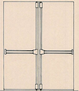
DOUBLE LEAF DOOR: 2 top and bottom latch type device
