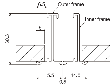
■ Sectional view of outer/inner frame
